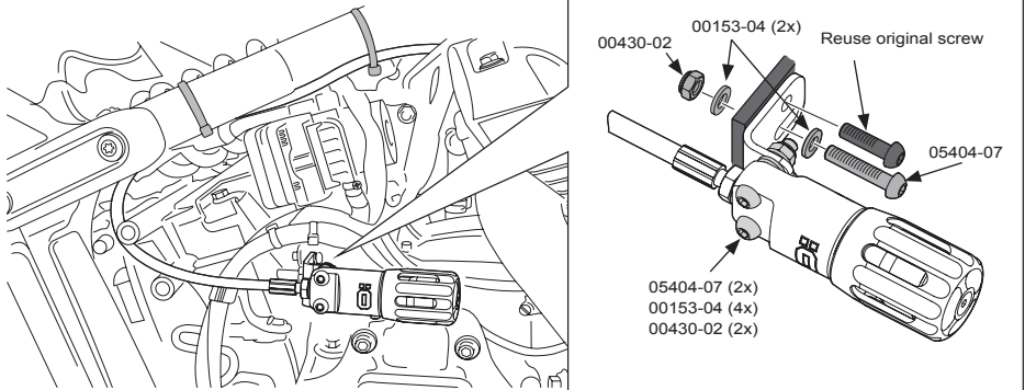
Fig. 2 - Mounting bracket option for HD 505LW (2018-22 Softail Lowrider, Deluxe, Slim, and Street Bob)
