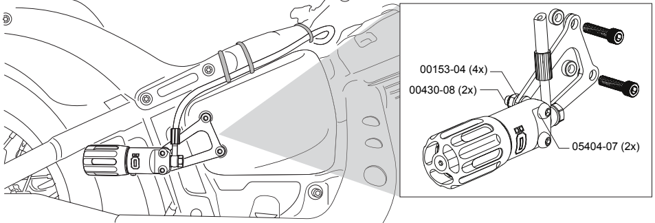
Fig. 2 - Mounting bracket option for HD 505LW (2018-22 Softail Lowrider, Deluxe, Slim, and Street Bob)
